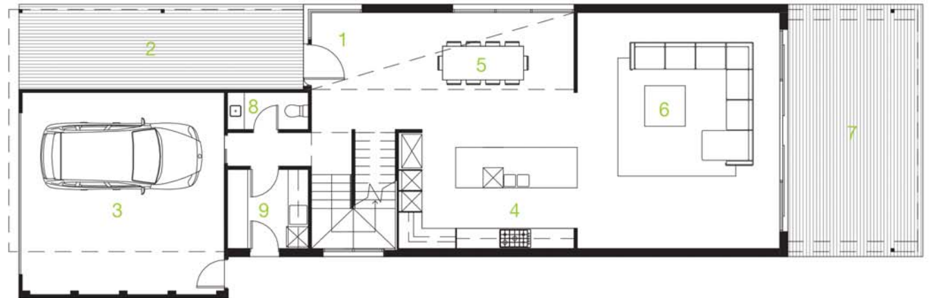
Ground Floor
